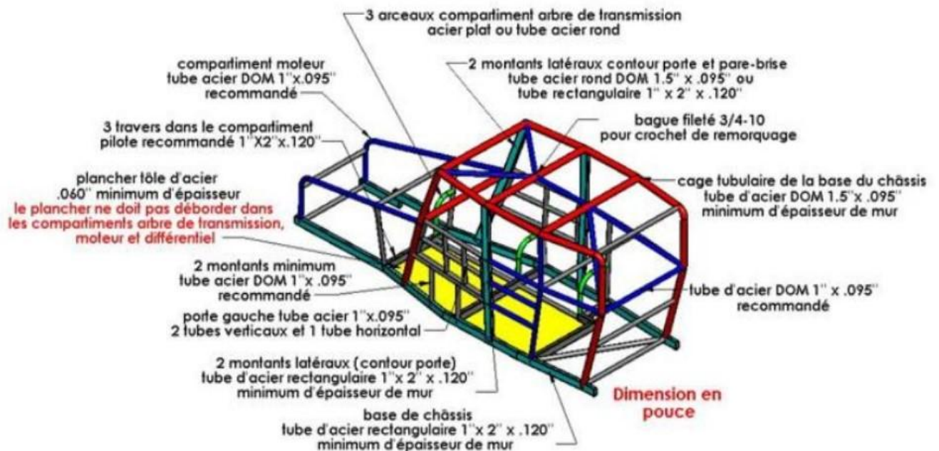
Figure 1 Châssis sedan
